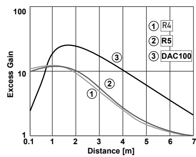
EXCESS GAIN
